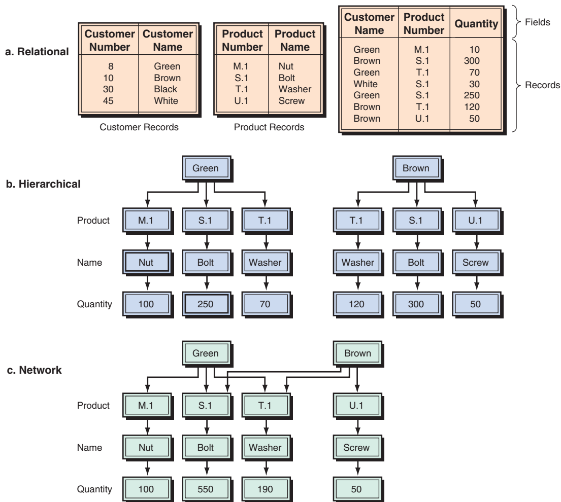
Figure T3.4 Database structures.
